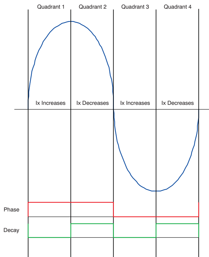
Figure 9. Decay Mode
