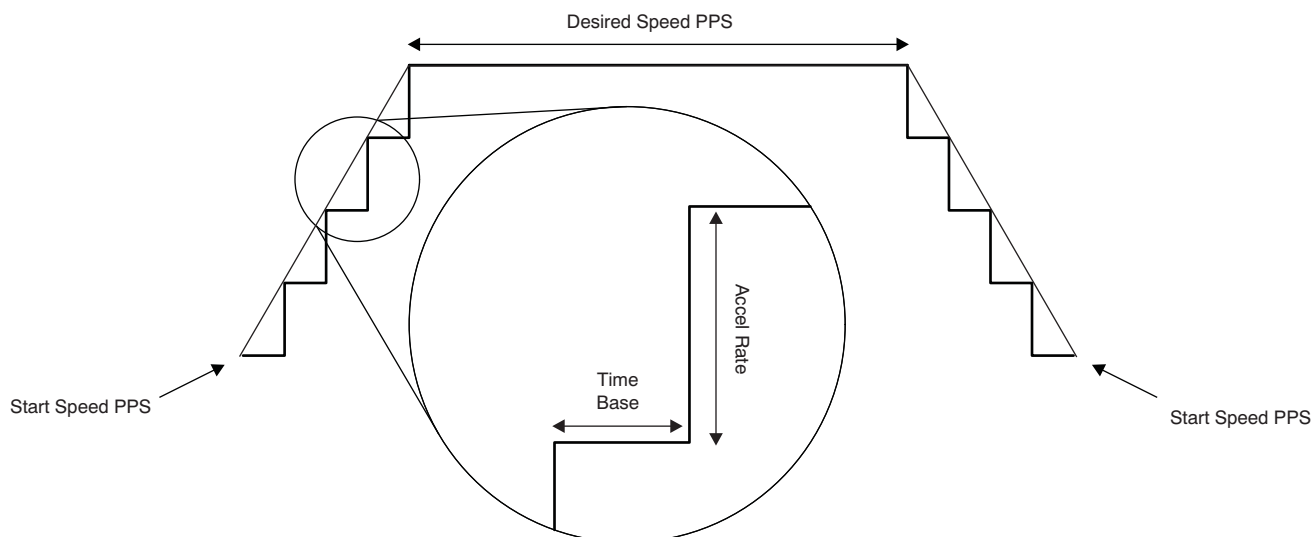
Figure 8. Acceleration Profile
